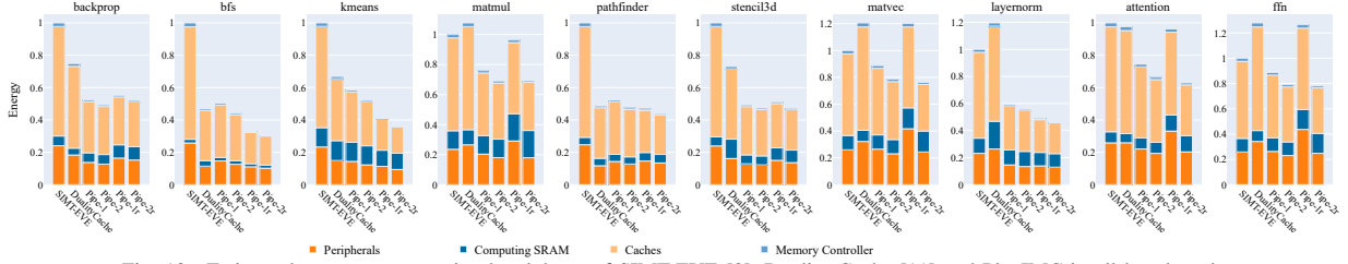
Fig. 10. Estimated energy consumption breakdown of SIMT-EVE [2], Duality Cache [11] and PipeIMC in all benchmarks.
